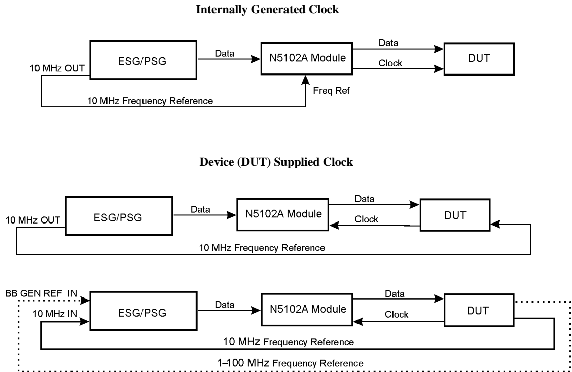
Figure 11-3 Frequency Reference Setup Diagrams for the N5102A Module Clock Signal
